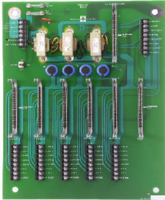
MR-50 Module Rack, 115 VAC 51009011 $1,200
